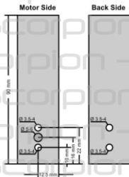
Horizontal Roll Motor Tube (2)
