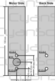
Tilt Motor Tube (1)
